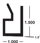
8" Stackable SF Retainer x 24' 6" 24-63-405 (MO)
