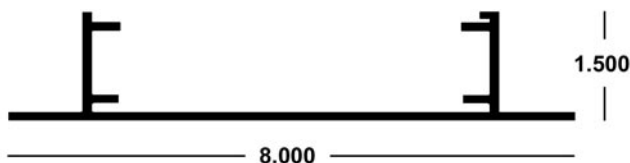
8" Stackable Sign Frame x 24' 6" 24-63-400 (MO) Corner Key: 1/8" Angles
