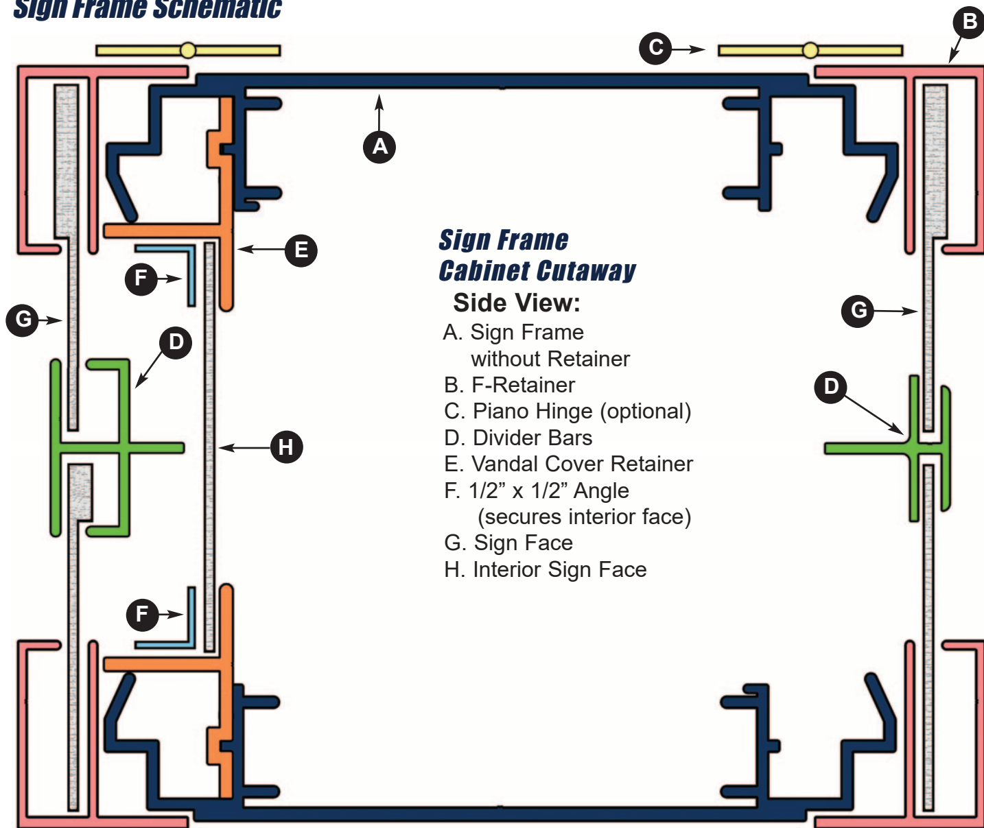
8" Stackable Sign Frame x 24' 6" 24-63-400 (MO) Corner Key: 1/8" Angles
