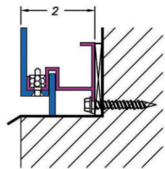
SILL DETAIL
