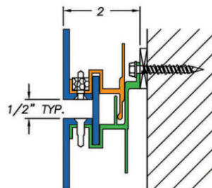
HORIZONTAL JOINT DETAIL
