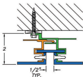
VERTICAL JOINT DETAIL
