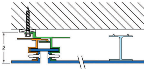
VERTICAL JOINT SHOWING STIFFENER
