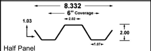
Half Panel
