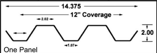
One Panel
